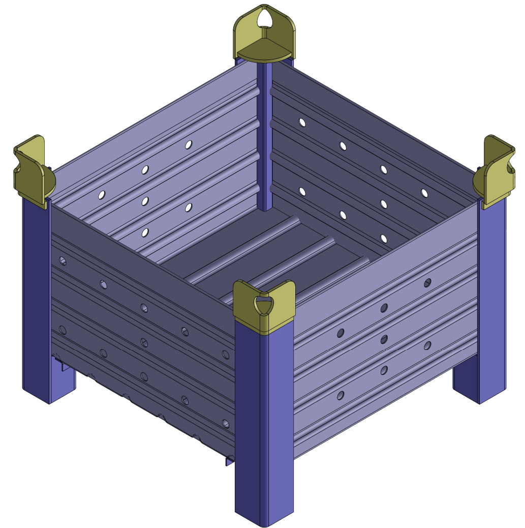
ISOMETRIC VIEW
